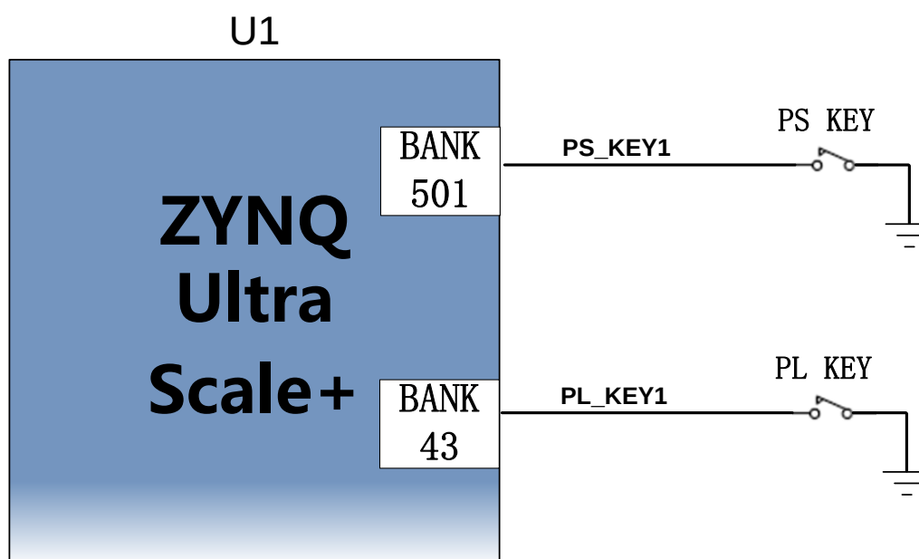
Figure 3-16-1: Rest keys connection diagram
